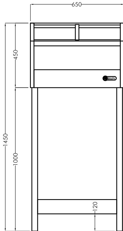
VISTA FRONTAL
